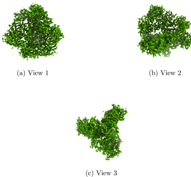
Figure 4: Isosurface at threshold=0.097000. Views generated by ChimeraX at a the following X, Y, Z angles: View 1 (0, -90, -90), View 2 (-90, 0, -90), View 3 (0, 0, 0).
