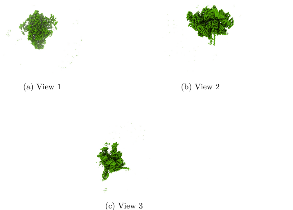
Figure 4: Isosurface at threshold=0.116000. Views generated by ChimeraX at a the following X, Y, Z angles: View 1 (0, -90, -90), View 2 (-90, 0, -90), View 3 (0, 0, 0).
