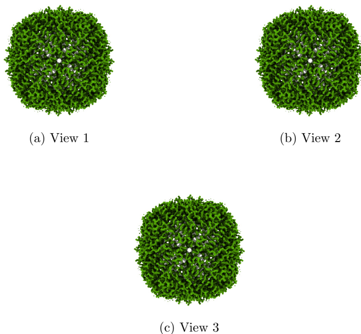
Figure 4: Isosurface at threshold=0.009530. Views generated by ChimeraX at a the following X, Y, Z angles: View 1 (0, -90, -90), View 2 (-90, 0, -90), View 3 (0, 0, 0).
