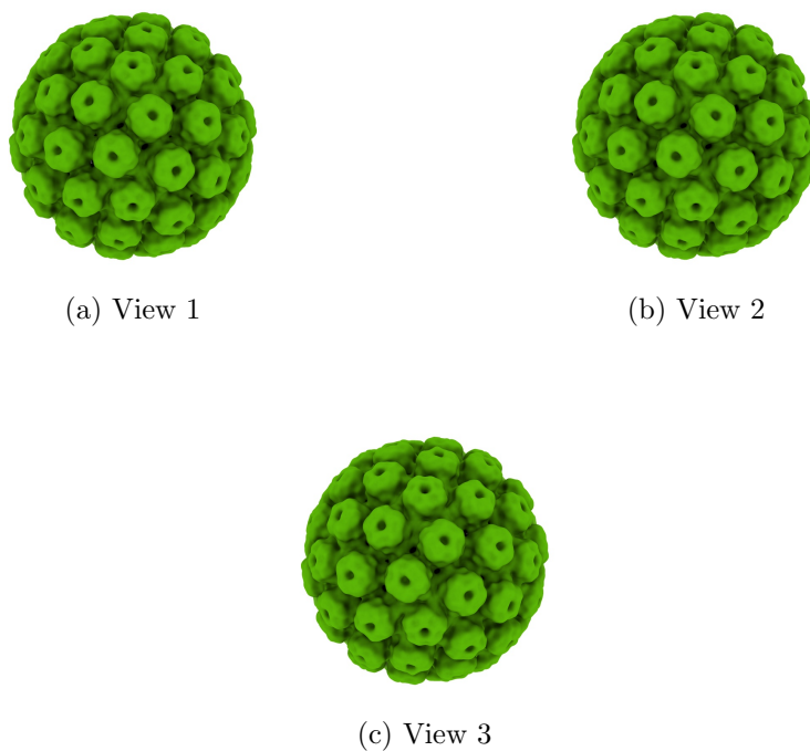
Figure 4: Isosurface at threshold=26.000000. Views generated by ChimeraX at a the following X, Y, Z angles: View 1 (0, -90, -90), View 2 (-90, 0, -90), View 3 (0, 0, 0).
