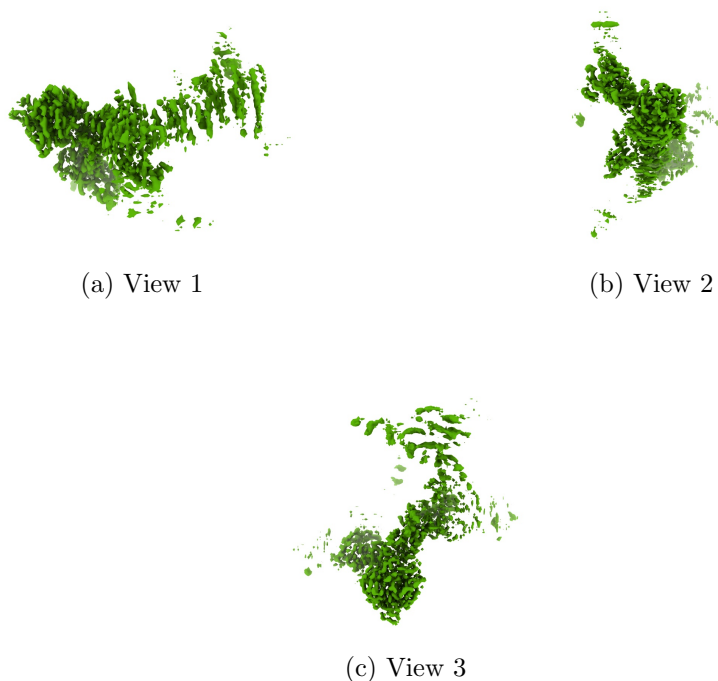
Figure 4: Isosurface at threshold=0.204000. Views generated by ChimeraX at a the following X, Y, Z angles: View 1 (0, -90, -90), View 2 (-90, 0, -90), View 3 (0, 0, 0).
