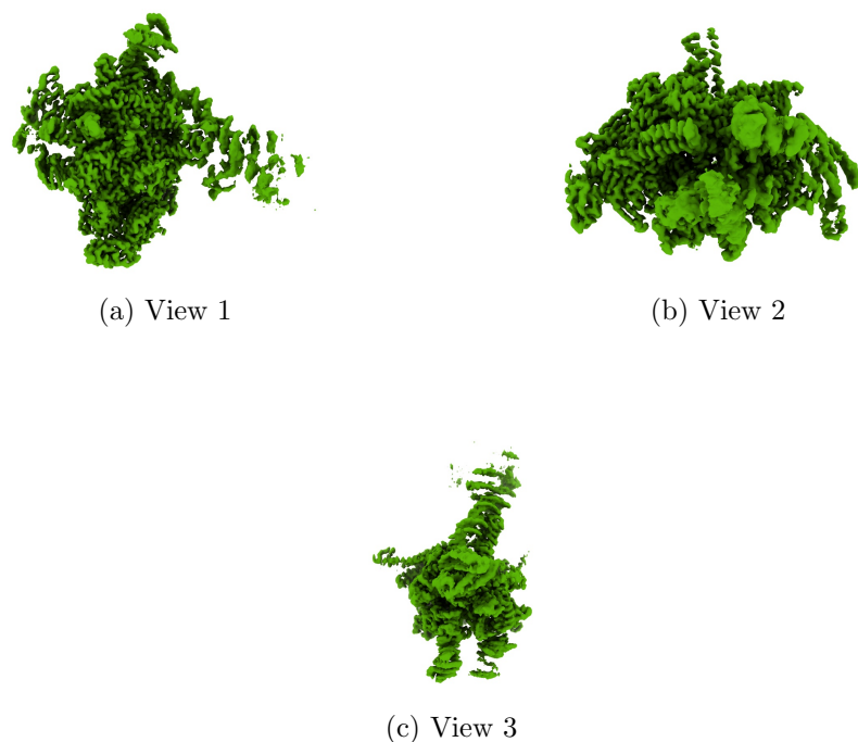
Figure 4: Isosurface at threshold=0.069400. Views generated by ChimeraX at a the following X, Y, Z angles: View 1 (0, -90, -90), View 2 (-90, 0, -90), View 3 (0, 0, 0).
