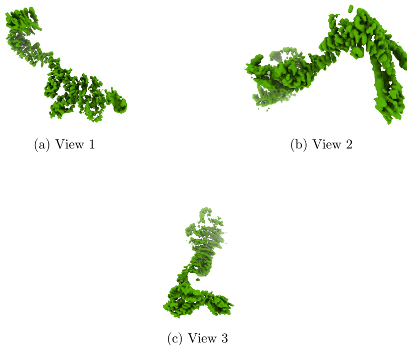
Figure 4: Isosurface at threshold=0.081800. Views generated by ChimeraX at a the following X, Y, Z angles: View 1 (0, -90, -90), View 2 (-90, 0, -90), View 3 (0, 0, 0).
