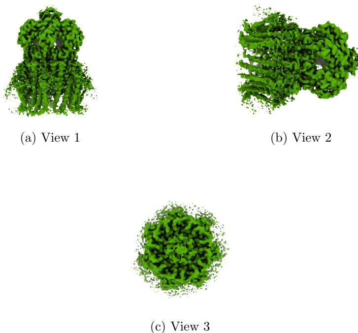
Figure 4: Isosurface at threshold=4.500000. Views generated by ChimeraX at a the following X, Y, Z angles: View 1 (0, -90, -90), View 2 (-90, 0, -90), View 3 (0, 0, 0).
