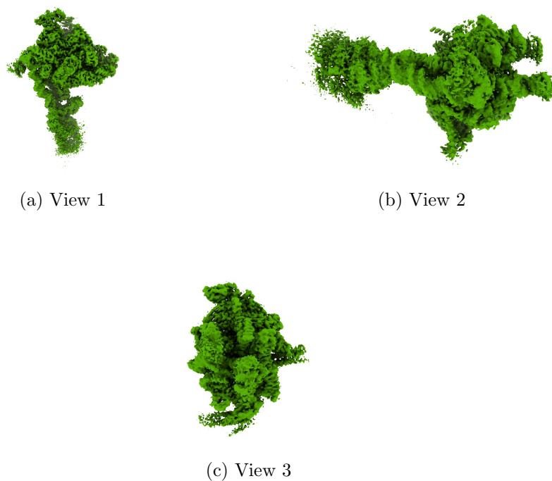
Figure 4: Isosurface at threshold=0.002370. Views generated by ChimeraX at a the following X, Y, Z angles: View 1 (0, -90, -90), View 2 (-90, 0, -90), View 3 (0, 0, 0).
