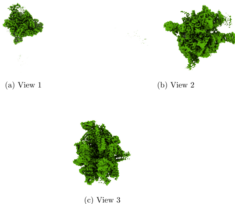
Figure 4: Isosurface at threshold=0.003210. Views generated by ChimeraX at a the following X, Y, Z angles: View 1 (0, -90, -90), View 2 (-90, 0, -90), View 3 (0, 0, 0).
