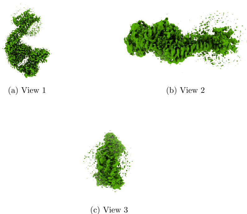
Figure 4: Isosurface at threshold=0.067100. Views generated by ChimeraX at a the following X, Y, Z angles: View 1 (0, -90, -90), View 2 (-90, 0, -90), View 3 (0, 0, 0).
