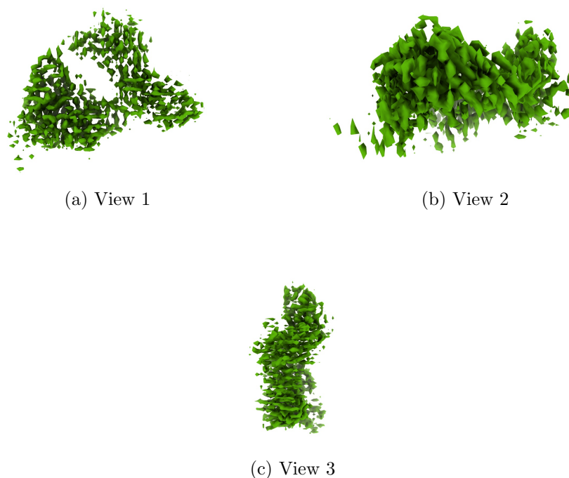
Figure 4: Isosurface at threshold=0.156000. Views generated by ChimeraX at a the following X, Y, Z angles: View 1 (0, -90, -90), View 2 (-90, 0, -90), View 3 (0, 0, 0).
