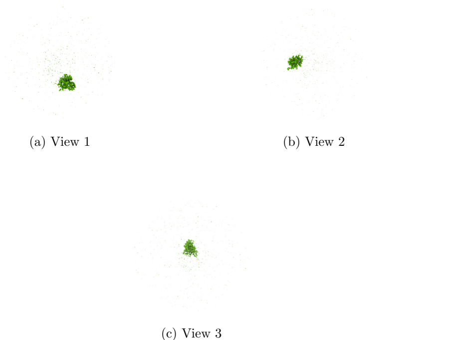
Figure 4: Isosurface at threshold=0.109000. Views generated by ChimeraX at a the following X, Y, Z angles: View 1 (0, -90, -90), View 2 (-90, 0, -90), View 3 (0, 0, 0).
