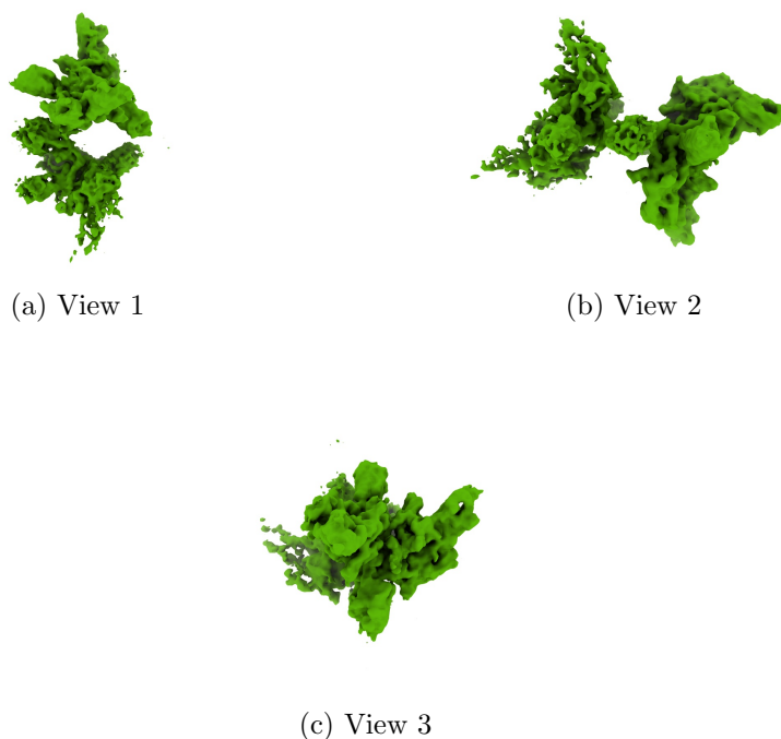
Figure 4: Isosurface at threshold=0.142000. Views generated by ChimeraX at a the following X, Y, Z angles: View 1 (0, -90, -90), View 2 (-90, 0, -90), View 3 (0, 0, 0).
