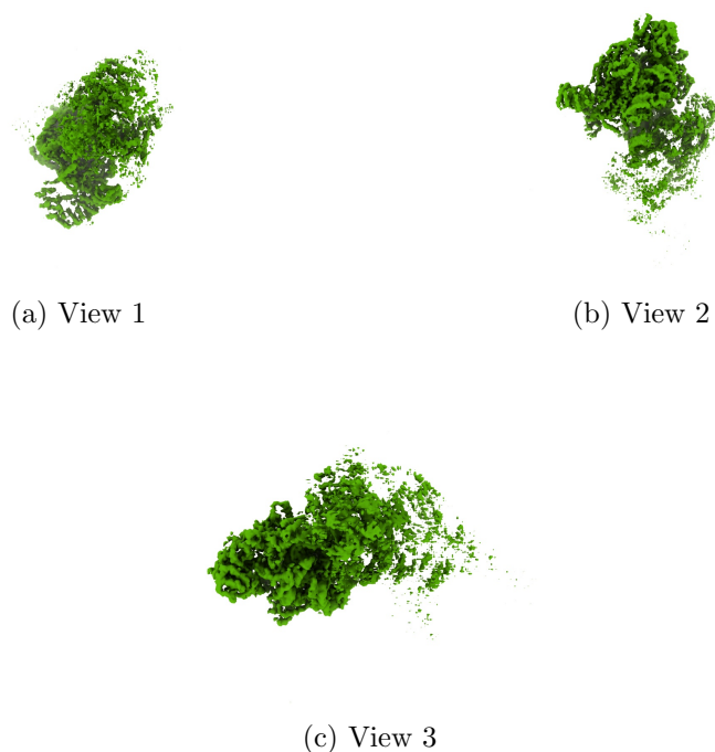
Figure 4: Isosurface at threshold=0.379000. Views generated by ChimeraX at a the following X, Y, Z angles: View 1 (0, -90, -90), View 2 (-90, 0, -90), View 3 (0, 0, 0).
