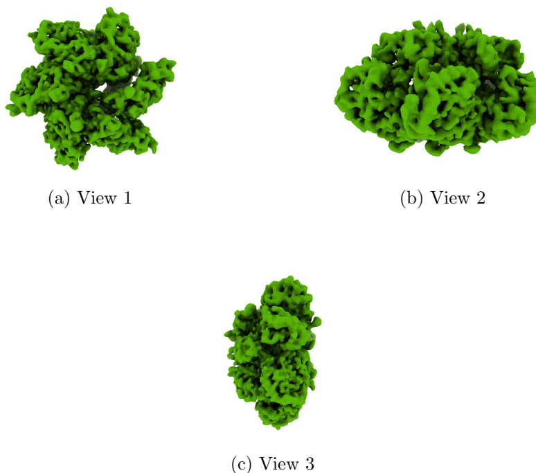
Figure 4: Isosurface at threshold=3.150000. Views generated by ChimeraX at a the following X, Y, Z angles: View 1 (0, -90, -90), View 2 (-90, 0, -90), View 3 (0, 0, 0).
