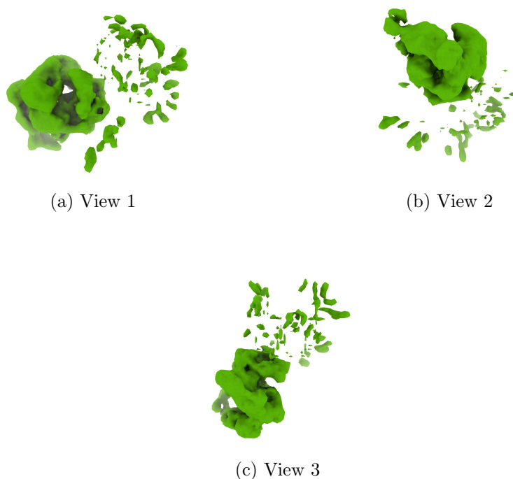
Figure 4: Isosurface at threshold=0.566000. Views generated by ChimeraX at a the following X, Y, Z angles: View 1 (0, -90, -90), View 2 (-90, 0, -90), View 3 (0, 0, 0).
