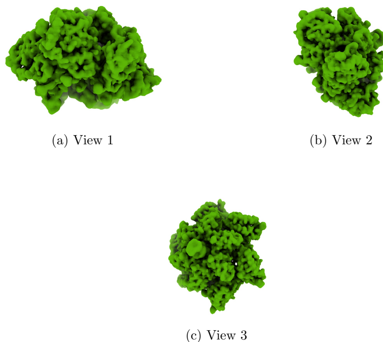
Figure 4: Isosurface at threshold=2.290000. Views generated by ChimeraX at a the following X, Y, Z angles: View 1 (0, -90, -90), View 2 (-90, 0, -90), View 3 (0, 0, 0).
