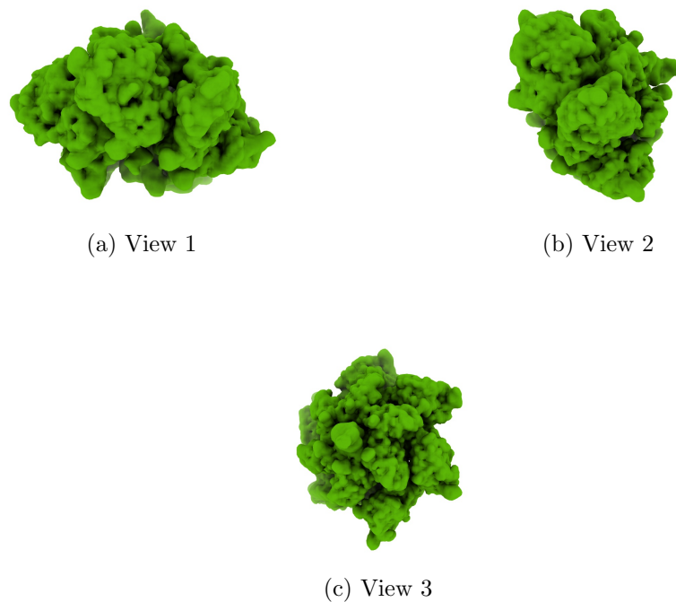
Figure 4: Isosurface at threshold=1.090000. Views generated by ChimeraX at a the following X, Y, Z angles: View 1 (0, -90, -90), View 2 (-90, 0, -90), View 3 (0, 0, 0).
