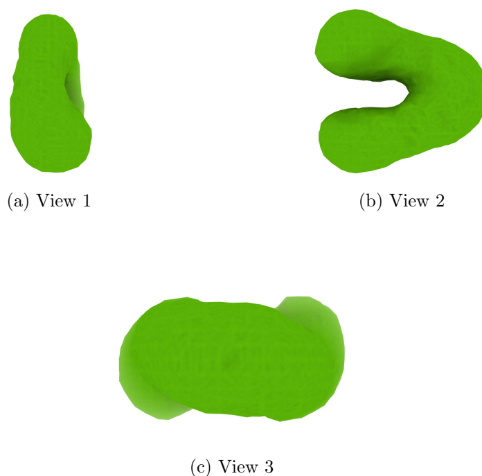
Figure 4: Isosurface at threshold=2.500000. Views generated by ChimeraX at a the following X, Y, Z angles: View 1 (0, -90, -90), View 2 (-90, 0, -90), View 3 (0, 0, 0).
