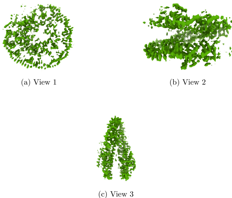
Figure 4: Isosurface at threshold=0.485000. Views generated by ChimeraX at a the following X, Y, Z angles: View 1 (0, -90, -90), View 2 (-90, 0, -90), View 3 (0, 0, 0).
