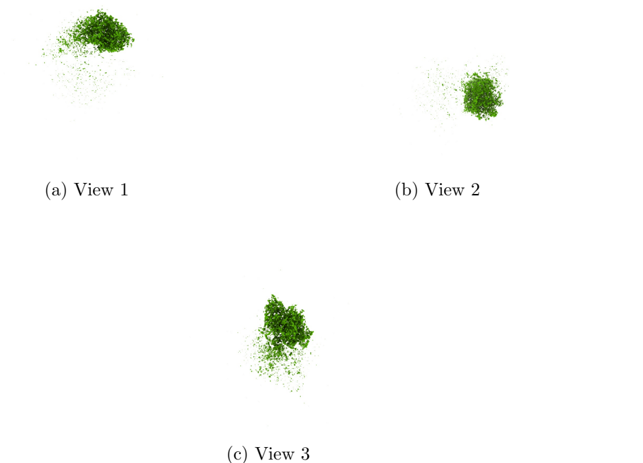
Figure 4: Isosurface at threshold=0.200000. Views generated by ChimeraX at a the following X, Y, Z angles: View 1 (0, -90, -90), View 2 (-90, 0, -90), View 3 (0, 0, 0).
