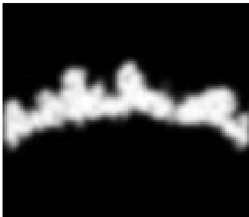
(a) X Slice 5
