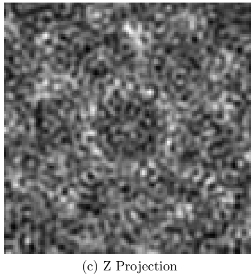
Figure 3: Projections in the three dimensions
