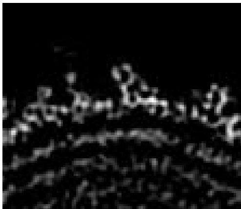
(a) X Slice 2
