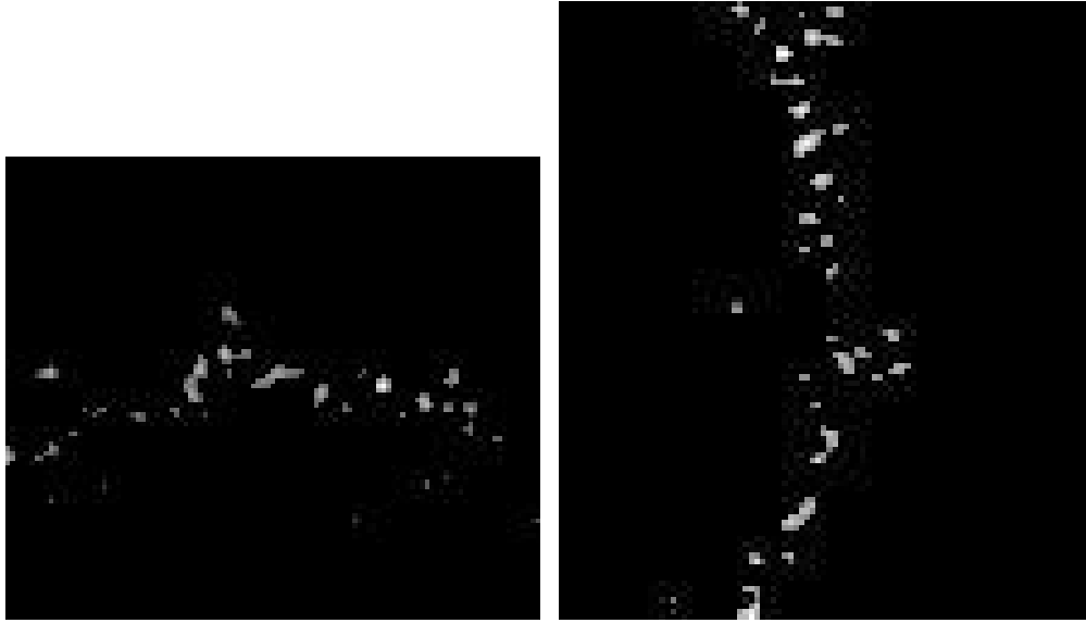
(a) X Slice 110
