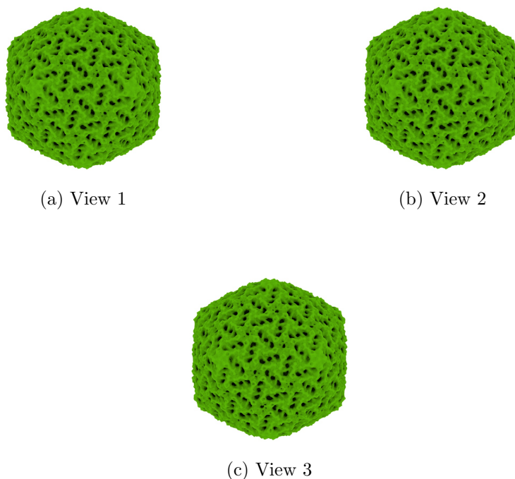
Figure 4: Isosurface at threshold=0.660000. Views generated by ChimeraX at a the following X, Y, Z angles: View 1 (0, -90, -90), View 2 (-90, 0, -90), View 3 (0, 0, 0).
