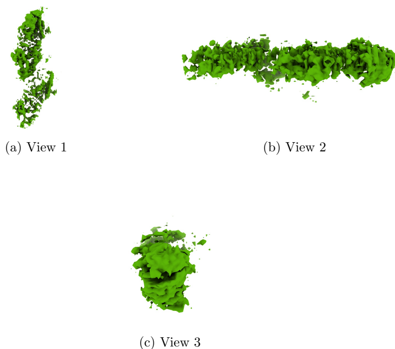
Figure 4: Isosurface at threshold=0.533000. Views generated by ChimeraX at a the following X, Y, Z angles: View 1 (0, -90, -90), View 2 (-90, 0, -90), View 3 (0, 0, 0).
