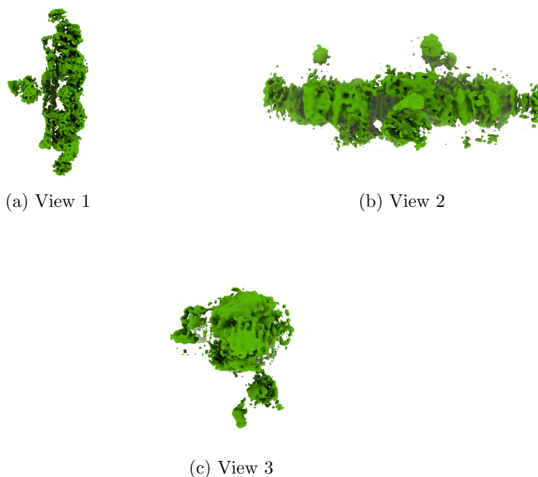
Figure 4: Isosurface at threshold=0.132000. Views generated by ChimeraX at a the following X, Y, Z angles: View 1 (0, -90, -90), View 2 (-90, 0, -90), View 3 (0, 0, 0).
