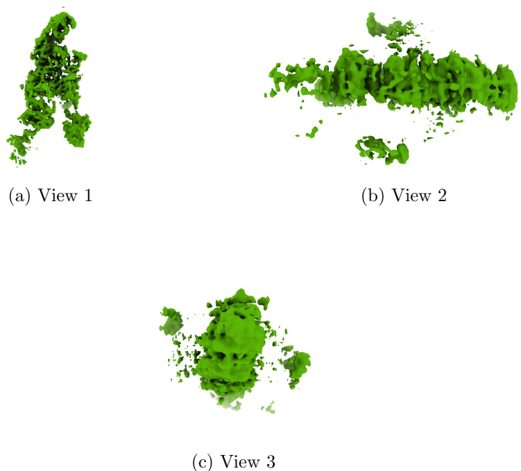
Figure 4: Isosurface at threshold=0.202000. Views generated by ChimeraX at a the following X, Y, Z angles: View 1 (0, -90, -90), View 2 (-90, 0, -90), View 3 (0, 0, 0).
