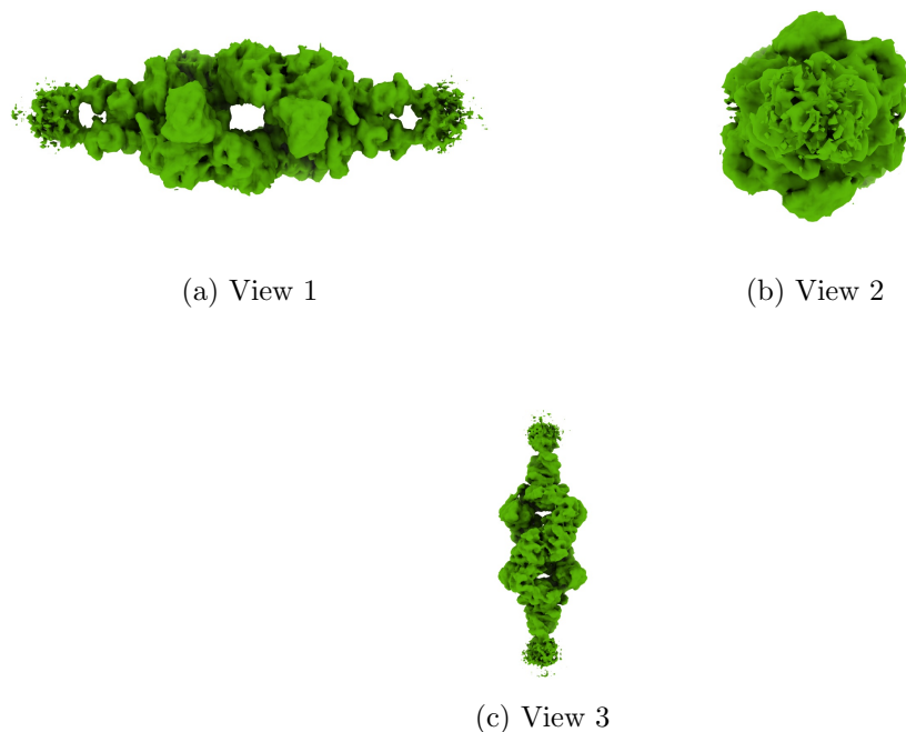
Figure 4: Isosurface at threshold=0.007000. Views generated by ChimeraX at a the following X, Y, Z angles: View 1 (0, -90, -90), View 2 (-90, 0, -90), View 3 (0, 0, 0).
