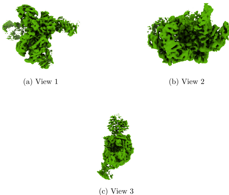
Figure 4: Isosurface at threshold=0.259000. Views generated by ChimeraX at a the following X, Y, Z angles: View 1 (0, -90, -90), View 2 (-90, 0, -90), View 3 (0, 0, 0).
