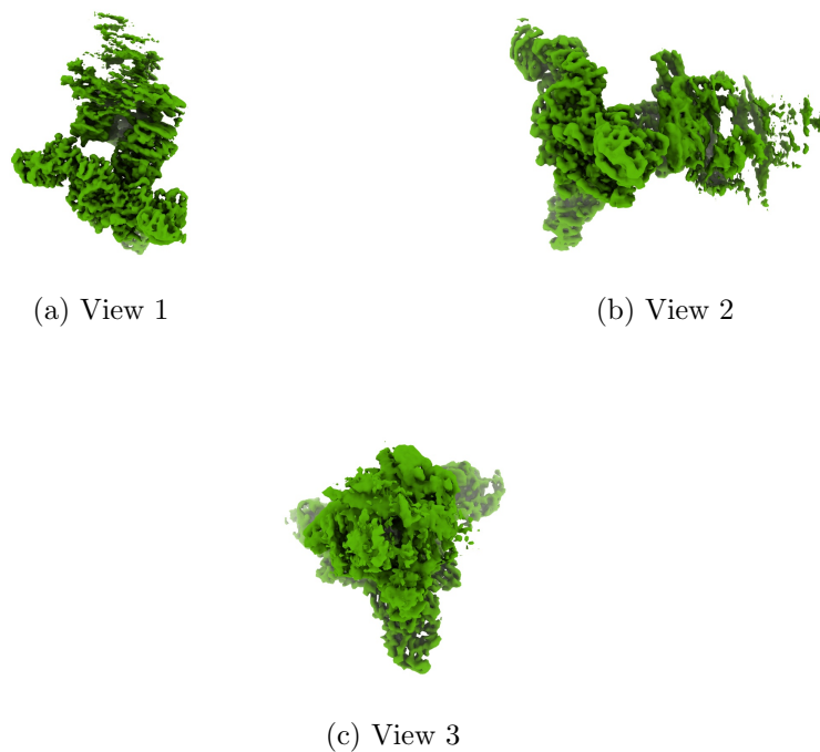
Figure 4: Isosurface at threshold=0.068900. Views generated by ChimeraX at a the following X, Y, Z angles: View 1 (0, -90, -90), View 2 (-90, 0, -90), View 3 (0, 0, 0).
