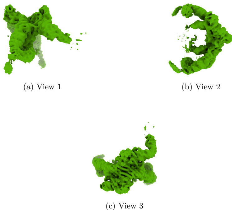
Figure 4: Isosurface at threshold=0.002280. Views generated by ChimeraX at a the following X, Y, Z angles: View 1 (0, -90, -90), View 2 (-90, 0, -90), View 3 (0, 0, 0).
