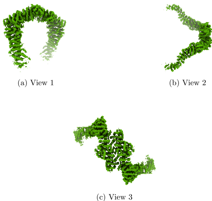
Figure 4: Isosurface at threshold=0.006680. Views generated by ChimeraX at a the following X, Y, Z angles: View 1 (0, -90, -90), View 2 (-90, 0, -90), View 3 (0, 0, 0).
