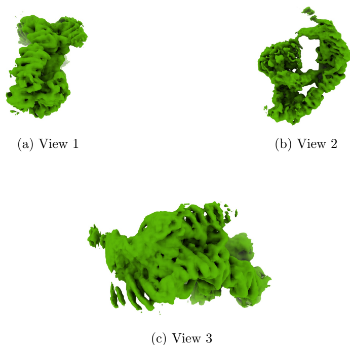
Figure 4: Isosurface at threshold=0.002650. Views generated by ChimeraX at a the following X, Y, Z angles: View 1 (0, -90, -90), View 2 (-90, 0, -90), View 3 (0, 0, 0).
