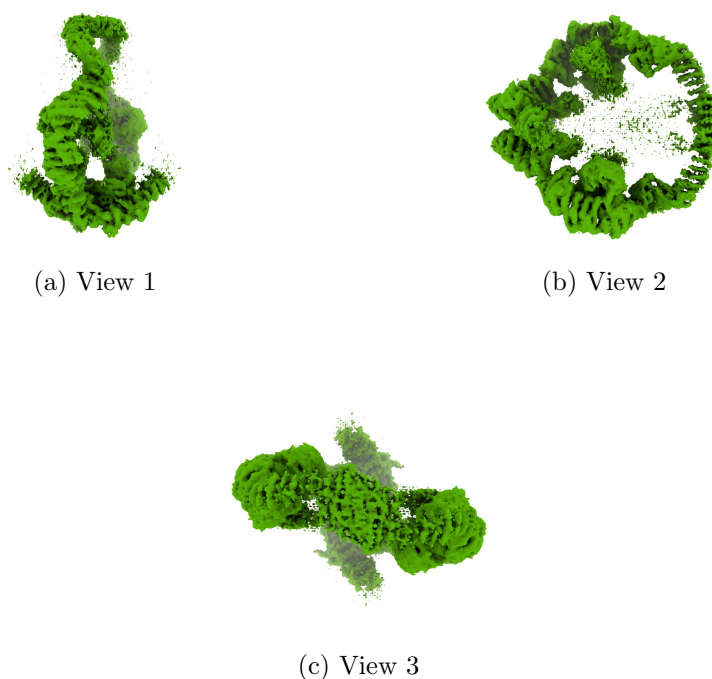
Figure 4: Isosurface at threshold=0.003440. Views generated by ChimeraX at a the following X, Y, Z angles: View 1 (0, -90, -90), View 2 (-90, 0, -90), View 3 (0, 0, 0).
