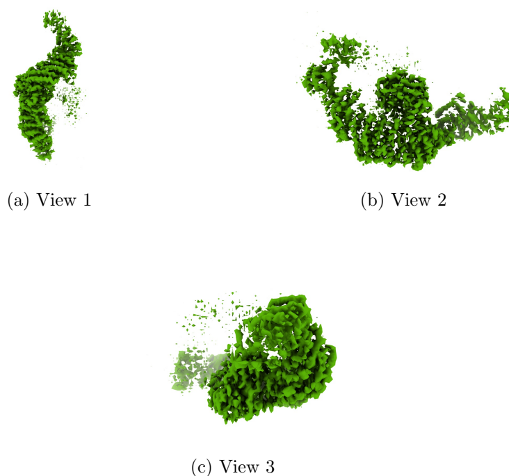
Figure 4: Isosurface at threshold=0.008400. Views generated by ChimeraX at a the following X, Y, Z angles: View 1 (0, -90, -90), View 2 (-90, 0, -90), View 3 (0, 0, 0).
