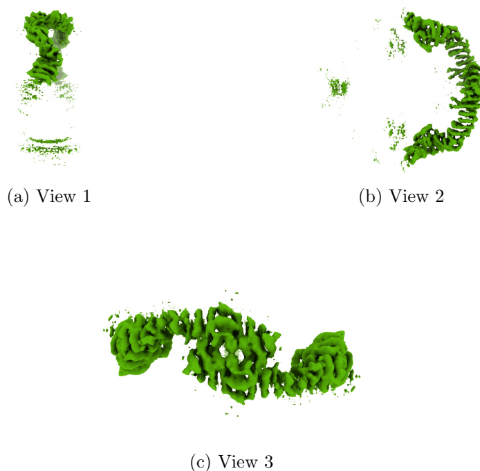
Figure 4: Isosurface at threshold=0.004500. Views generated by ChimeraX at a the following X, Y, Z angles: View 1 (0, -90, -90), View 2 (-90, 0, -90), View 3 (0, 0, 0).
