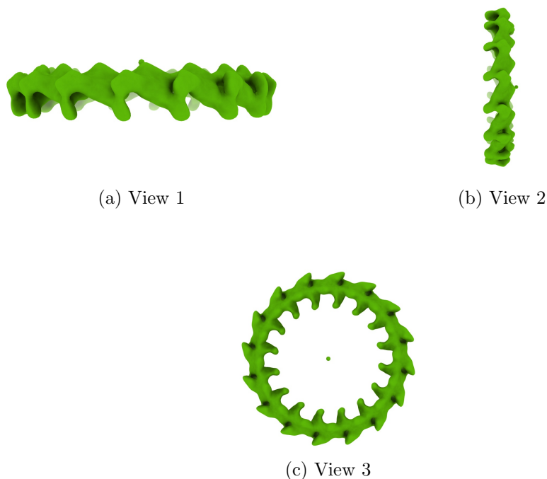
Figure 4: Isosurface at threshold=1.290000. Views generated by ChimeraX at a the following X, Y, Z angles: View 1 (0, -90, -90), View 2 (-90, 0, -90), View 3 (0, 0, 0).
