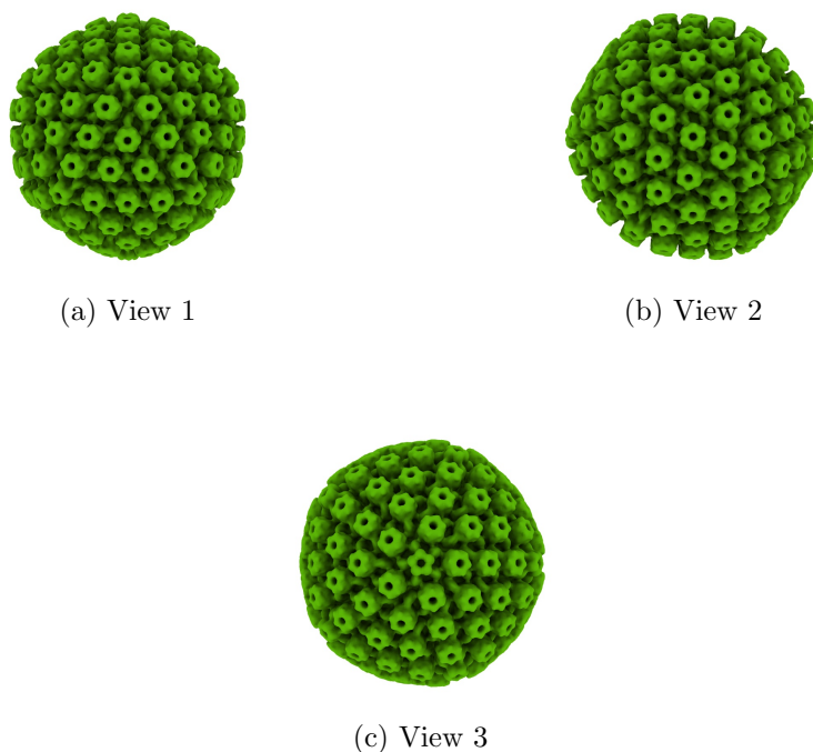
Figure 4: Isosurface at threshold=2.400000. Views generated by ChimeraX at a the following X, Y, Z angles: View 1 (0, -90, -90), View 2 (-90, 0, -90), View 3 (0, 0, 0).
