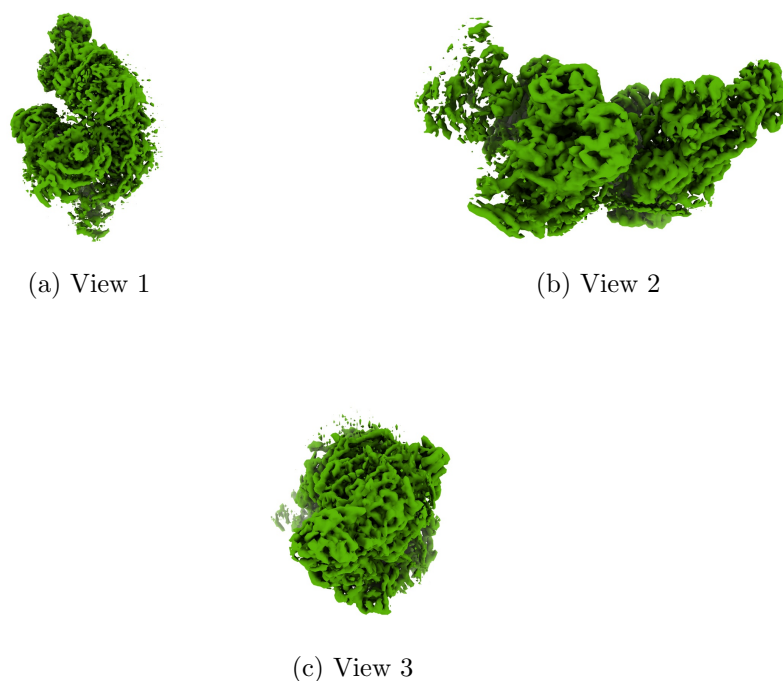
Figure 4: Isosurface at threshold=0.380000. Views generated by ChimeraX at a the following X, Y, Z angles: View 1 (0, -90, -90), View 2 (-90, 0, -90), View 3 (0, 0, 0).
