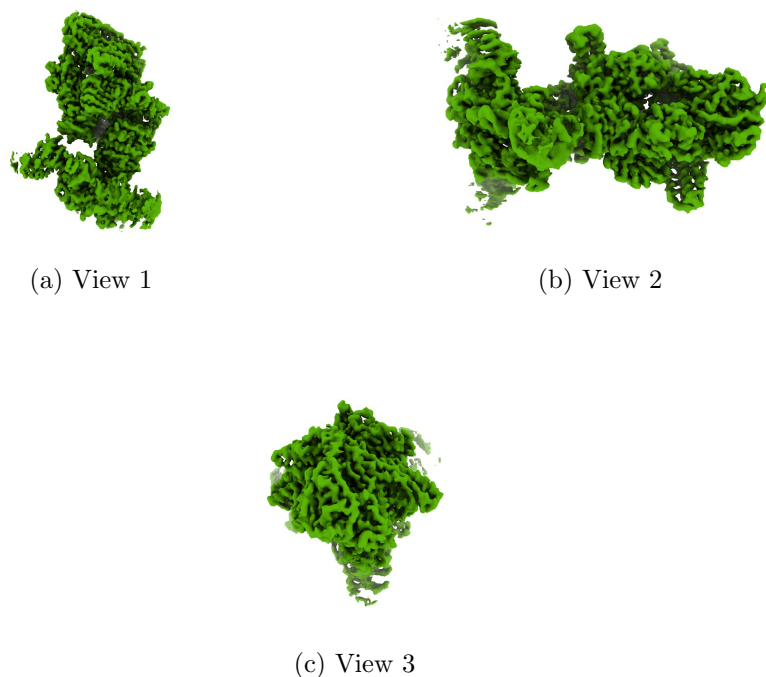
Figure 4: Isosurface at threshold=0.074000. Views generated by ChimeraX at a the following X, Y, Z angles: View 1 (0, -90, -90), View 2 (-90, 0, -90), View 3 (0, 0, 0).
