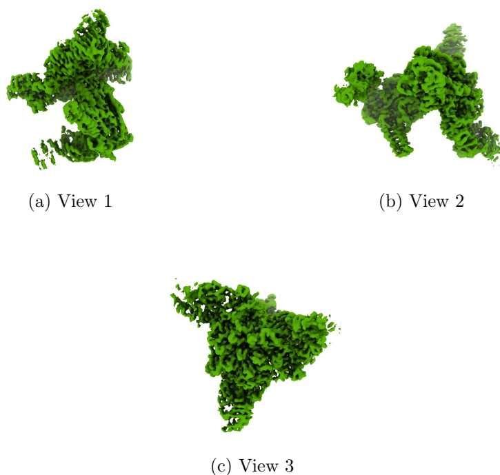
Figure 4: Isosurface at threshold=0.081100. Views generated by ChimeraX at a the following X, Y, Z angles: View 1 (0, -90, -90), View 2 (-90, 0, -90), View 3 (0, 0, 0).
