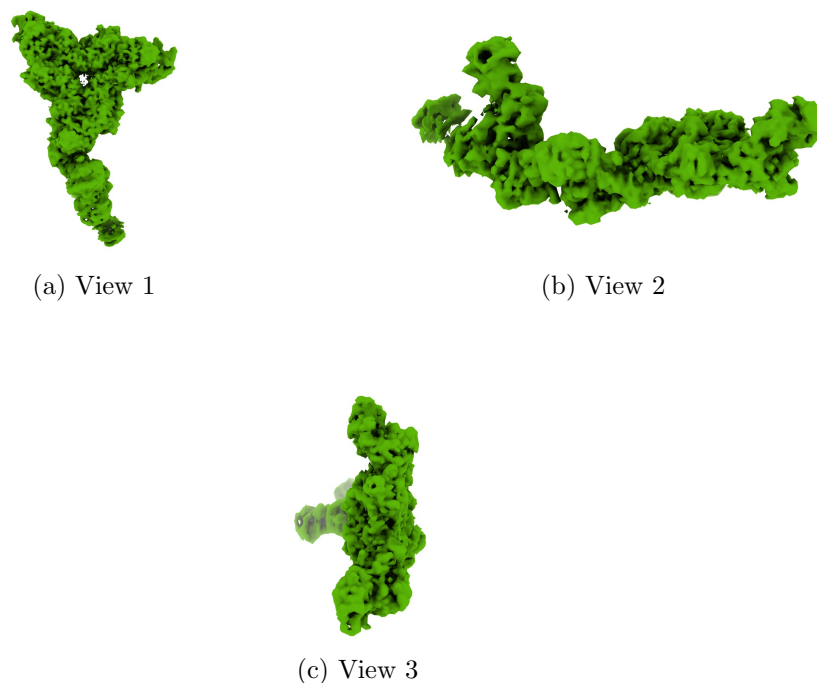
Figure 4: Isosurface at threshold=0.095900. Views generated by ChimeraX at a the following X, Y, Z angles: View 1 (0, -90, -90), View 2 (-90, 0, -90), View 3 (0, 0, 0).
