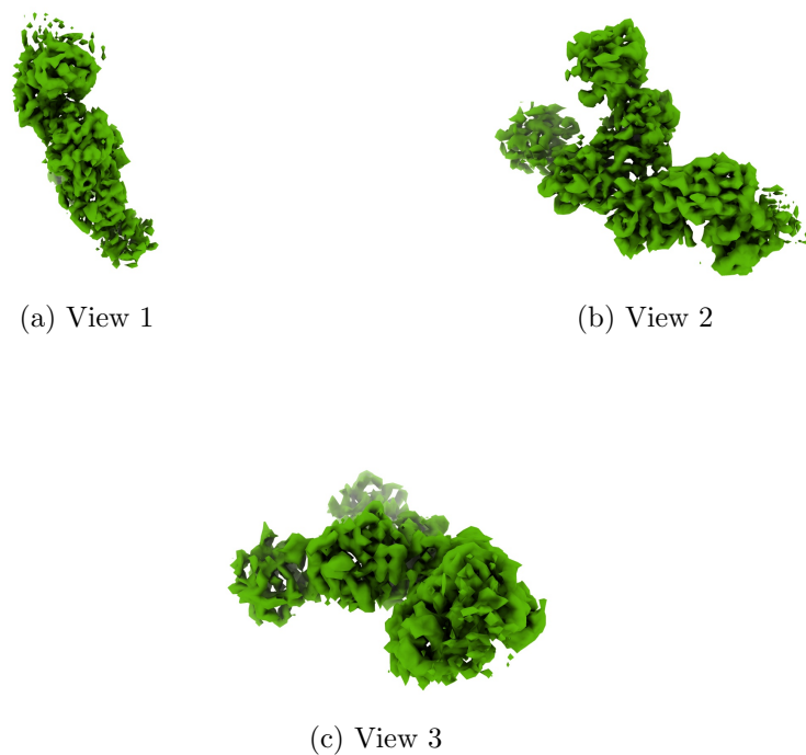
Figure 4: Isosurface at threshold=0.144000. Views generated by ChimeraX at a the following X, Y, Z angles: View 1 (0, -90, -90), View 2 (-90, 0, -90), View 3 (0, 0, 0).
