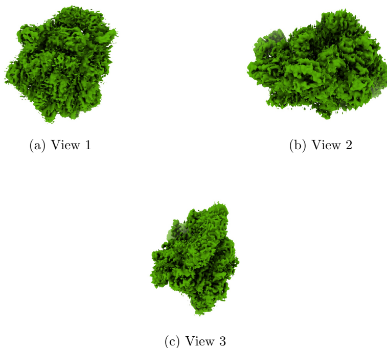
Figure 4: Isosurface at threshold=0.005000. Views generated by ChimeraX at the following X, Y, Z angles: View 1 (0, -90, -90), View 2 (-90, 0, -90), View 3 (0, 0, 0).
