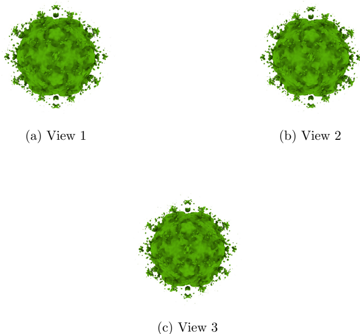
Figure 4: Isosurface at threshold=11.700000. Views generated by ChimeraX at a the following X, Y, Z angles: View 1 (0, -90, -90), View 2 (-90, 0, -90), View 3 (0, 0, 0).
