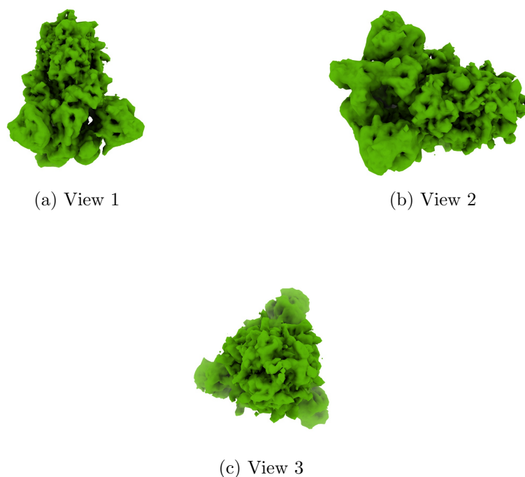
Figure 4: Isosurface at threshold=0.034000. Views generated by ChimeraX at a the following X, Y, Z angles: View 1 (0, -90, -90), View 2 (-90, 0, -90), View 3 (0, 0, 0).
