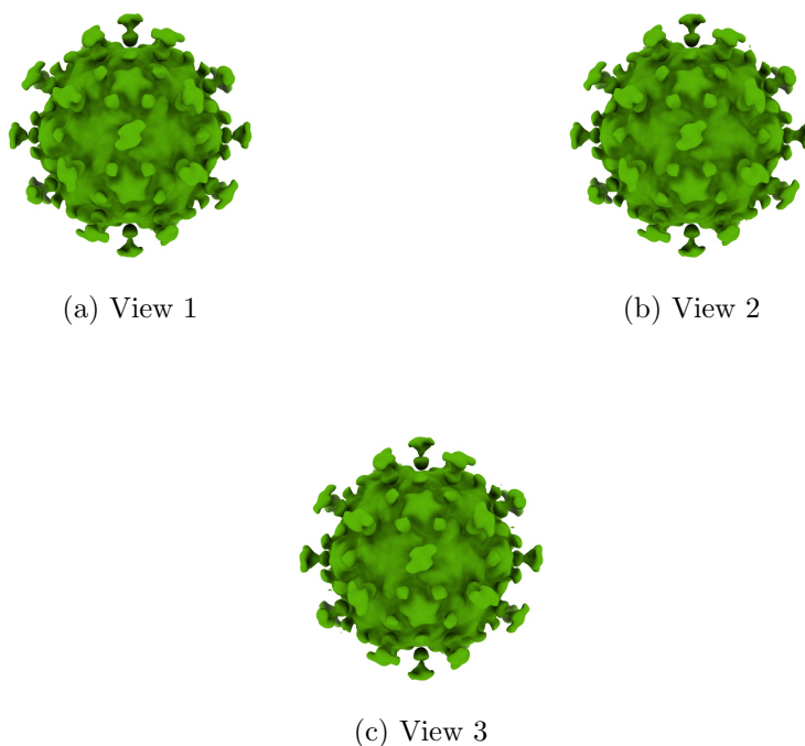
Figure 4: Isosurface at threshold=6.610000. Views generated by ChimeraX at a the following X, Y, Z angles: View 1 (0, -90, -90), View 2 (-90, 0, -90), View 3 (0, 0, 0).
