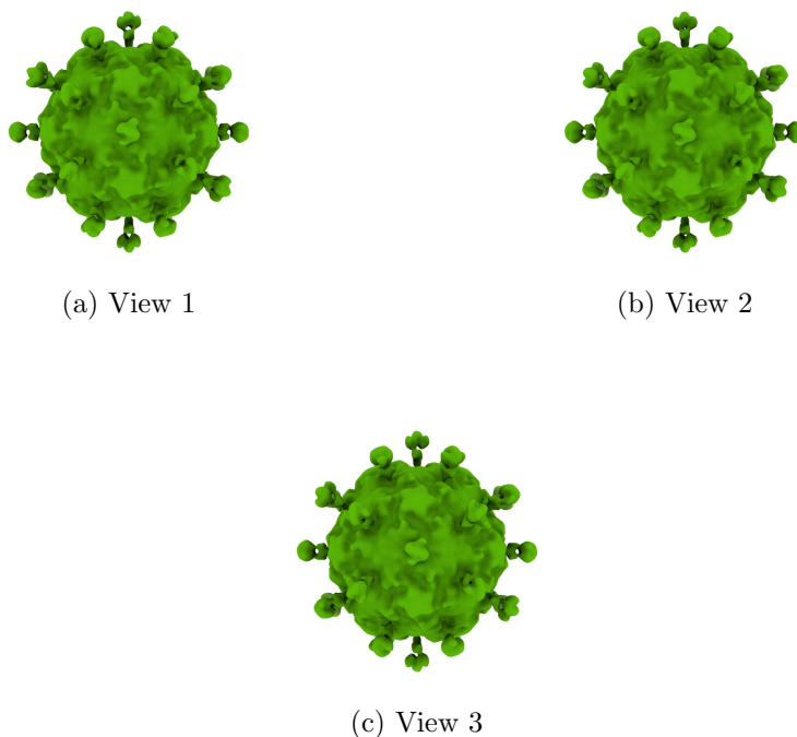
Figure 4: Isosurface at threshold=11.770000. Views generated by ChimeraX at a the following X, Y, Z angles: View 1 (0, -90, -90), View 2 (-90, 0, -90), View 3 (0, 0, 0).
