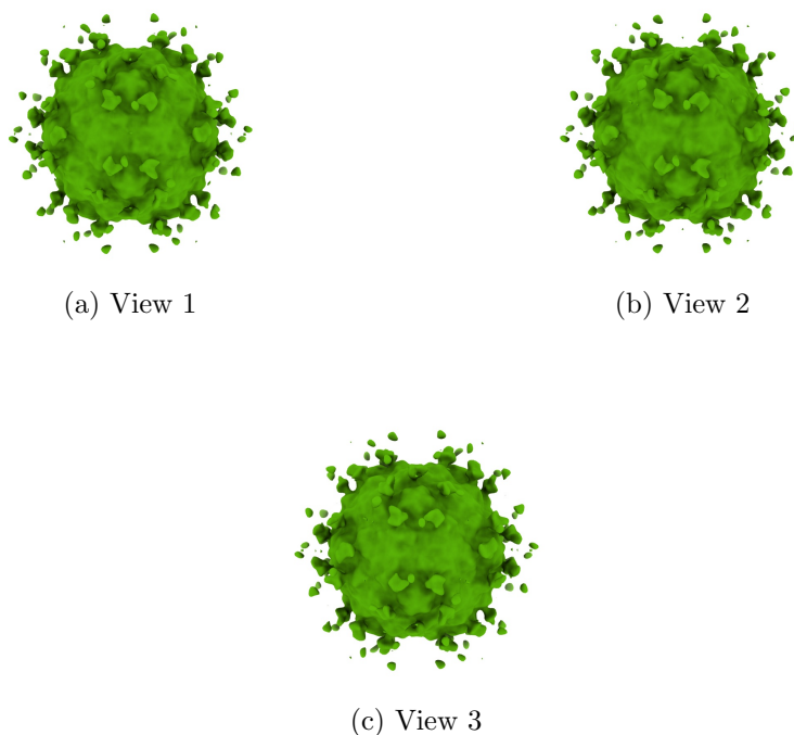
Figure 4: Isosurface at threshold=11.320000. Views generated by ChimeraX at a the following X, Y, Z angles: View 1 (0, -90, -90), View 2 (-90, 0, -90), View 3 (0, 0, 0).
