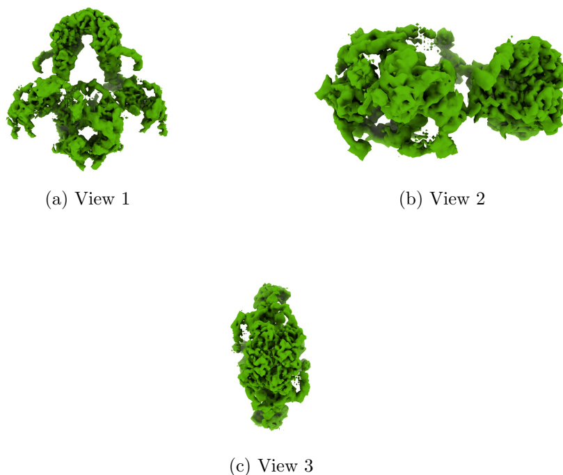
Figure 4: Isosurface at threshold=0.090000. Views generated by ChimeraX at the following X, Y, Z angles: View 1 (0, -90, -90), View 2 (-90, 0, -90), View 3 (0, 0, 0).
